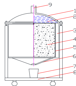
1-缸盖; 2-水; 3-缸筒; 4-试件; 5-止水缝材料; 6-有机玻璃漏斗; 7-量杯; 8-小车; 9-进水阀
